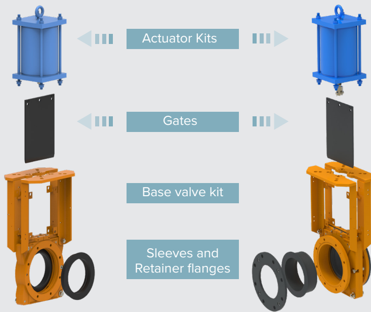
TGW valve model
