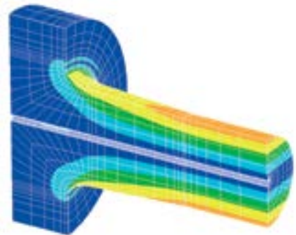
(Fig. 2) Stress applied to the new state-of-the-art design shows reduced stress concentration in critical area.
