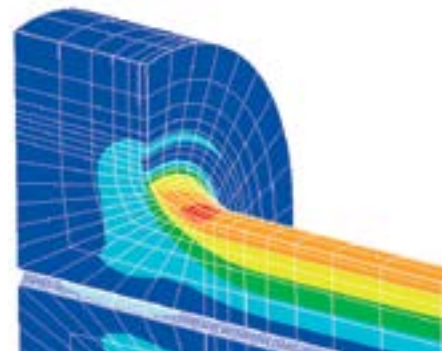
(Fig. 1) Stress applied to the traditional design shows increased stress concentration (in red) in critical area.
